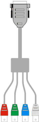
Figure 2 RGB to DVI(/VGA) Converter
